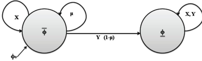
Fig. 2: \tilde{\Xi}^a automaton for the OLG game.
